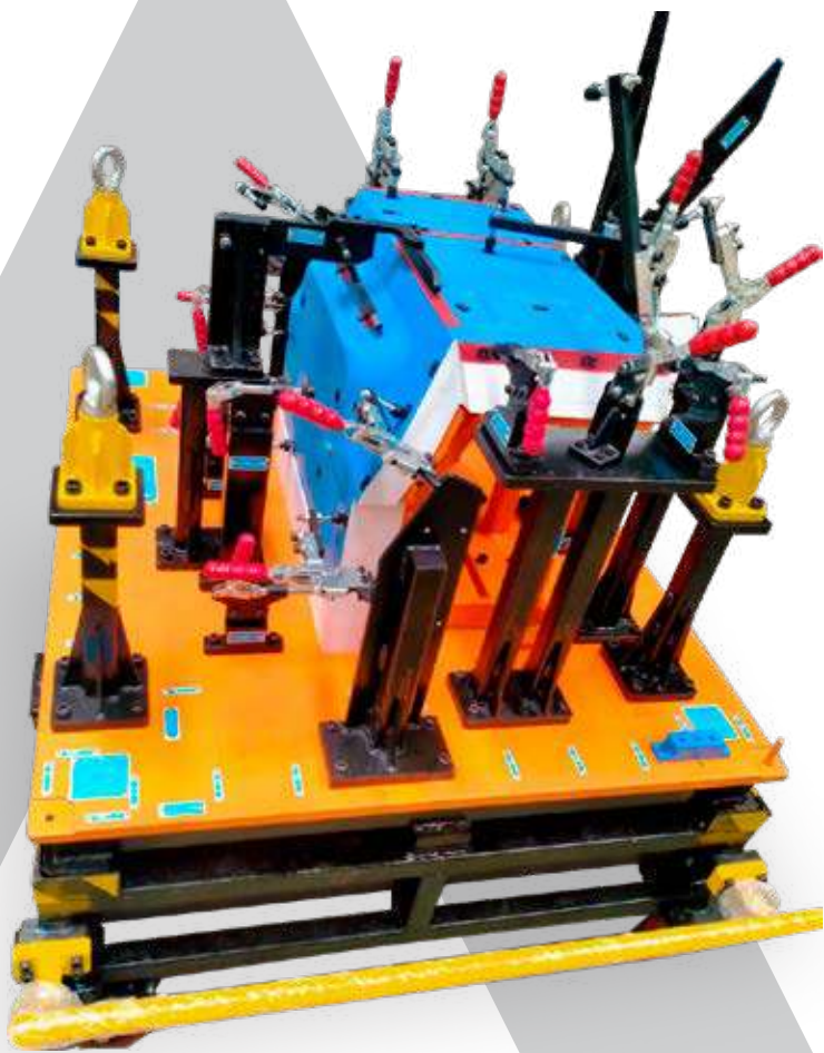
LH / RH Tow Panel Checking Fixture
